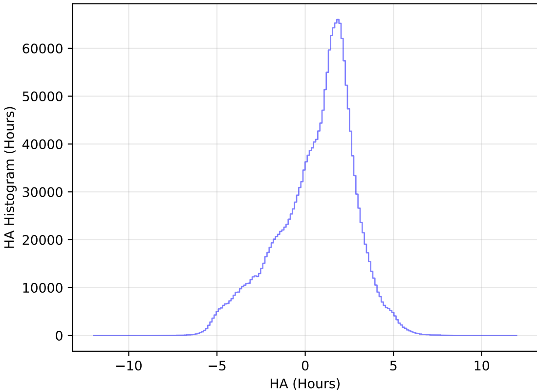
too_elab_r16_d3_gz_v3.4_10yrs All sky all bands: HA Histogram
