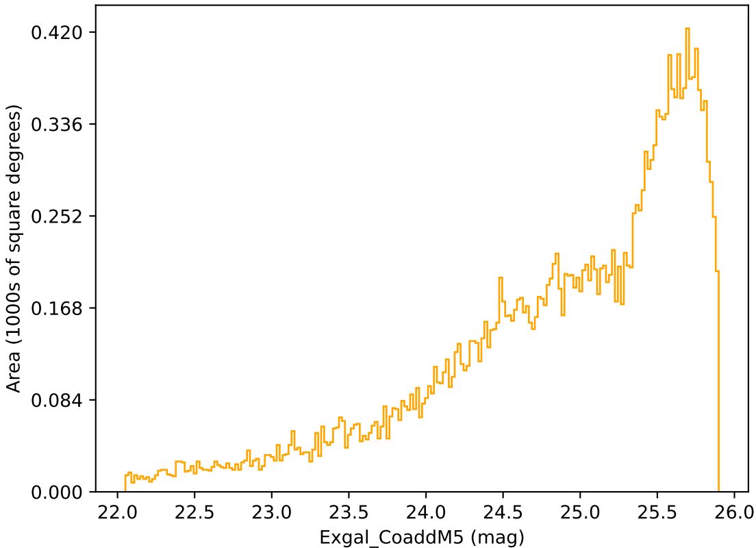
too_elab_r16_d3_gz_v3.4_10yrs Yr 3-4 r band: Exgal_CoaddM5
