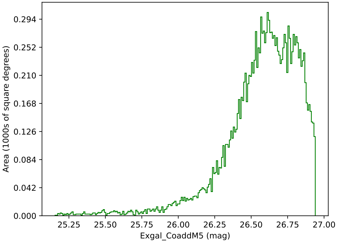
too_elab_r16_d3_gz_v3.4_10yrs WFD g band: Exgal_CoaddM5
