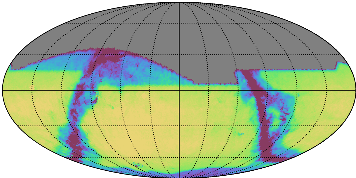
too_elab_r16_d3_gz_v3.4_10yrs All sky z band: Exgal_CoaddM5
