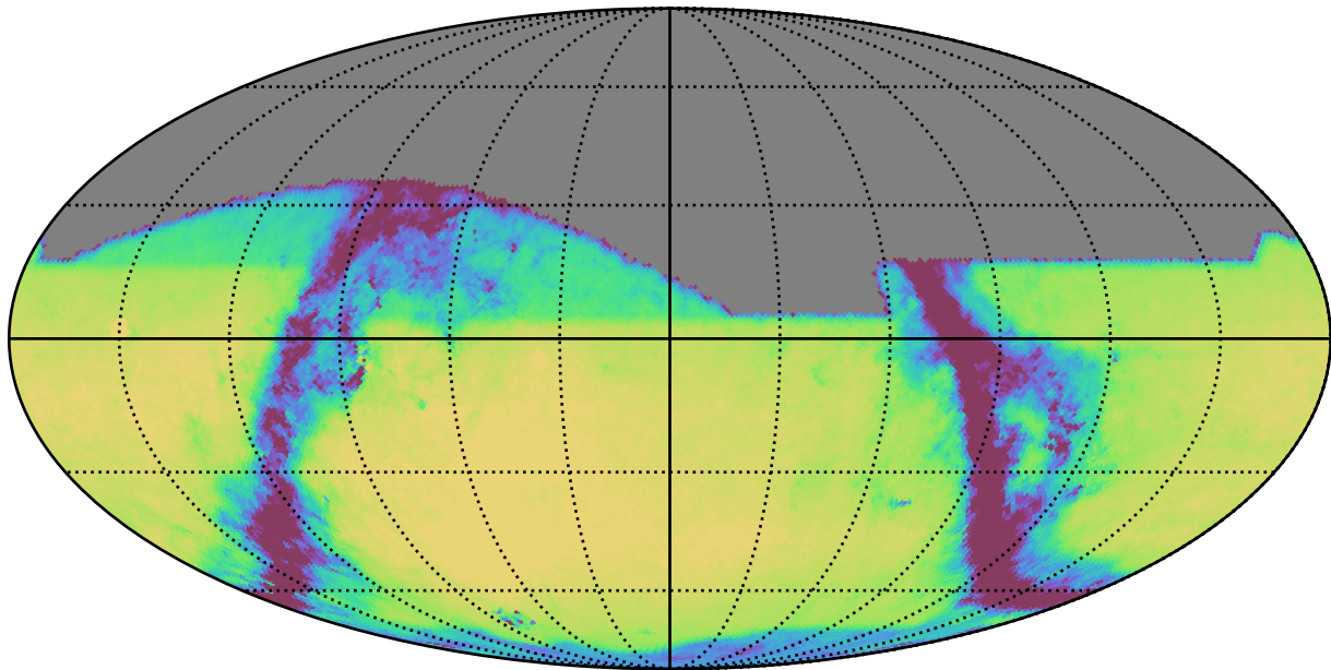
too_elab_r16_d3_gz_v3.4_10yrs All sky r band: Exgal_CoaddM5
