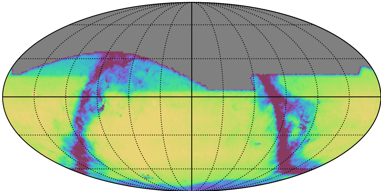
too_elab_r16_d3_gz_v3.4_10yrs All sky i band: Exgal_CoaddM5
