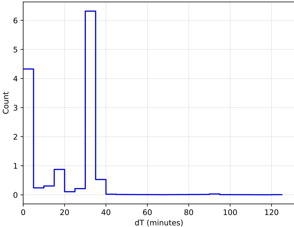
too_elab_r16_d3_gz_v3.4_10yrs All sky: DeltaT Histogram 1e6
