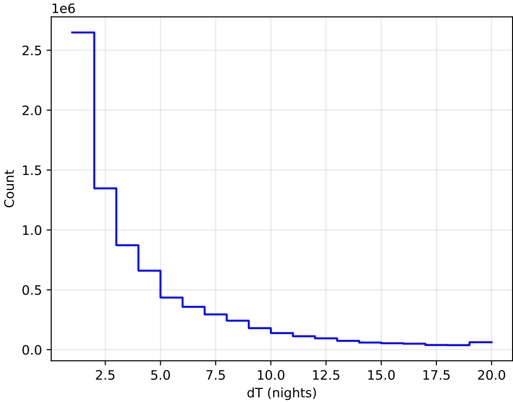
too_elab_r16_d3_gz_v3.4_10yrs WFD all bands: DeltaNight Histogram
