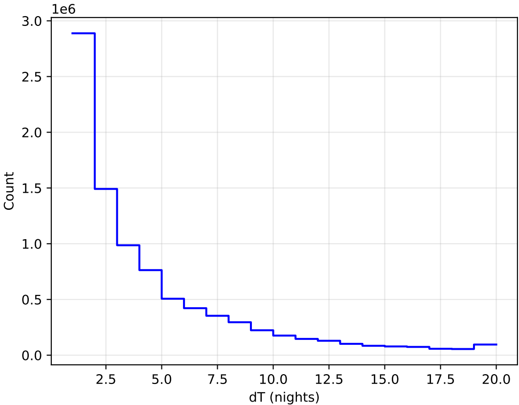
too_elab_r16_d3_gz_v3.4_10yrs All sky all bands: DeltaNight Histogram
