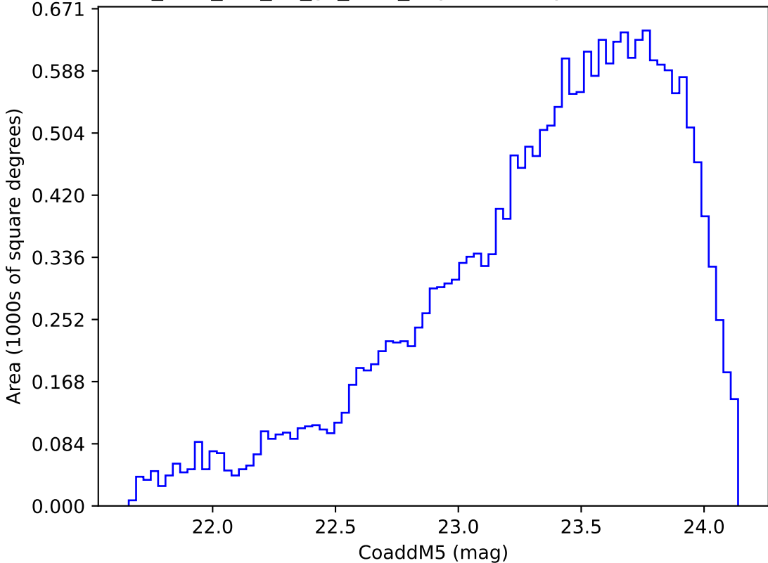
too_elab_r16_d3_gz_v3.4_10yrs Yr 3-4 y band: CoaddM5
