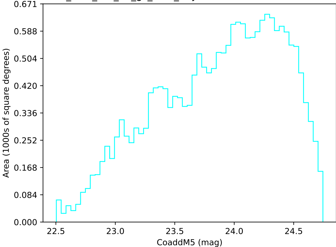
too_elab_r16_d3_gz_v3.4_10yrs Yr 3-4 u band: CoaddM5
