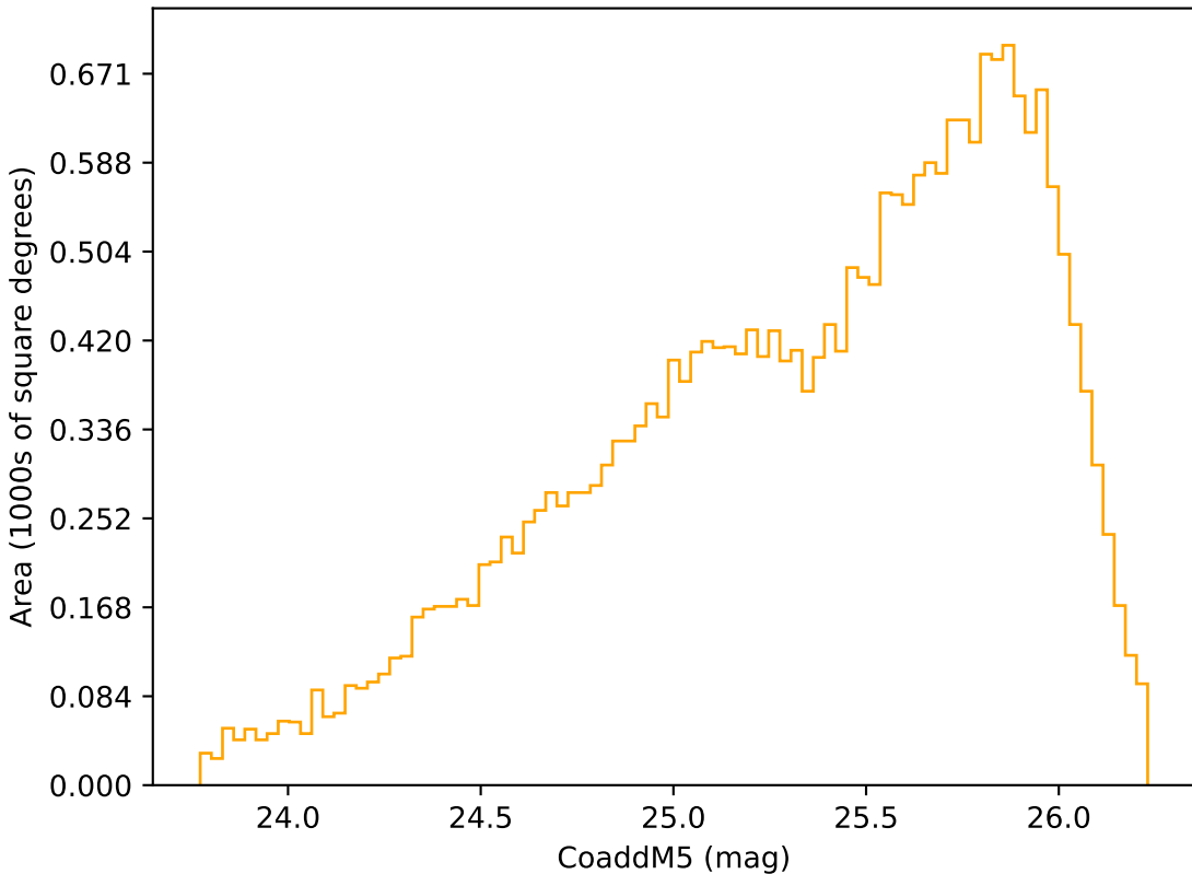
too_elab_r16_d3_gz_v3.4_10yrs Yr 3-4 r band: CoaddM5
