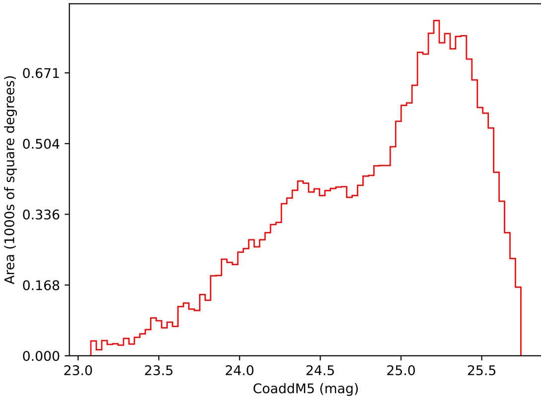
too_elab_r16_d3_gz_v3.4_10yrs Yr 3-4 i band: CoaddM5
