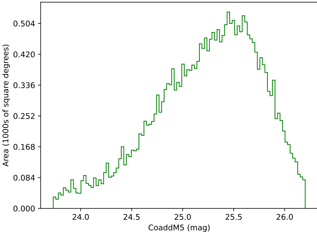
too_elab_r16_d3_gz_v3.4_10yrs Yr 3-4 g band: CoaddM5
