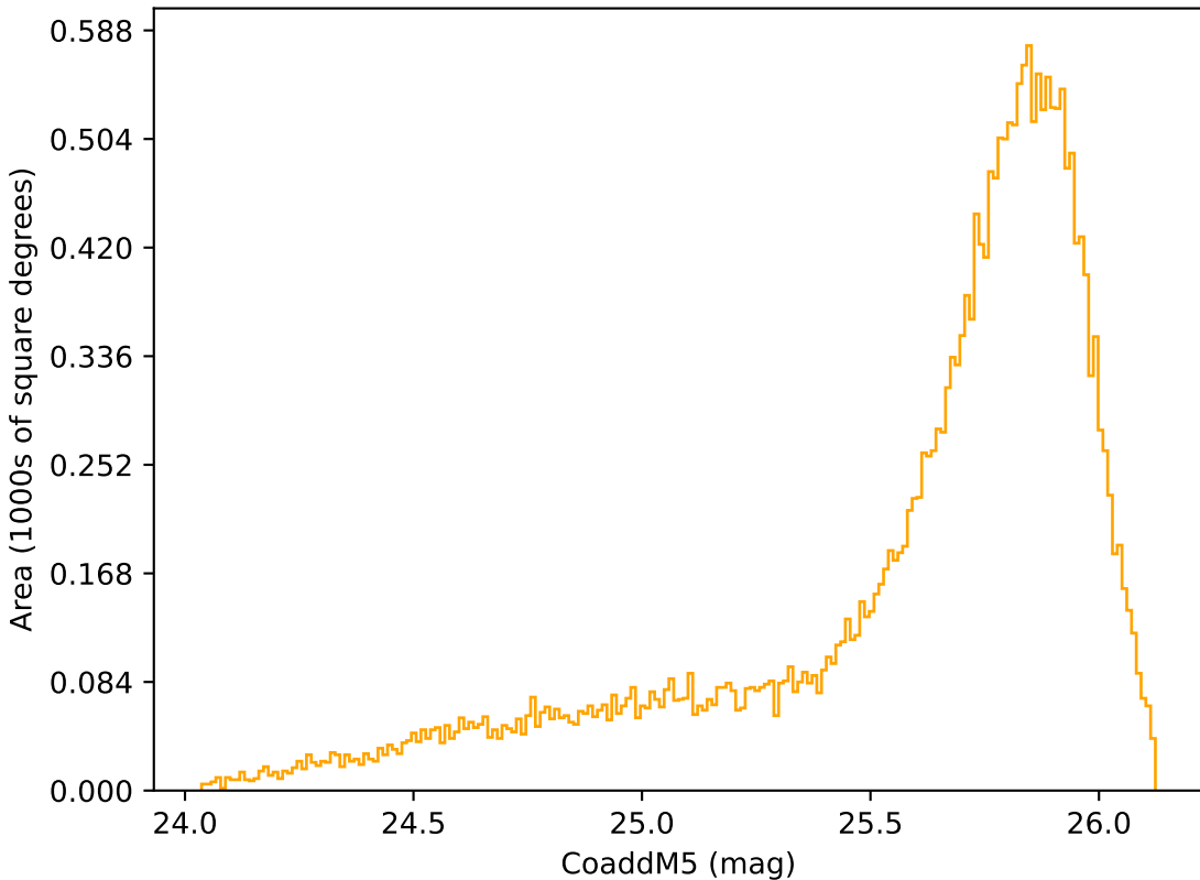
too_elab_r16_d3_gz_v3.4_10yrs Yr 1 r band: CoaddM5
