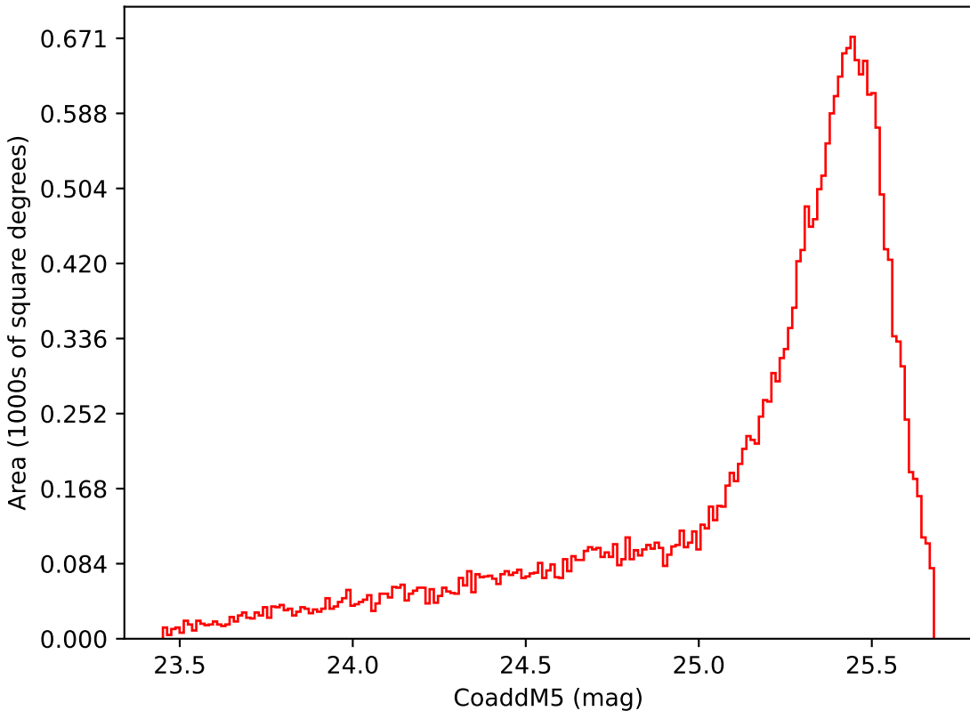
too_elab_r16_d3_gz_v3.4_10yrs Yr 1 i band: CoaddM5
