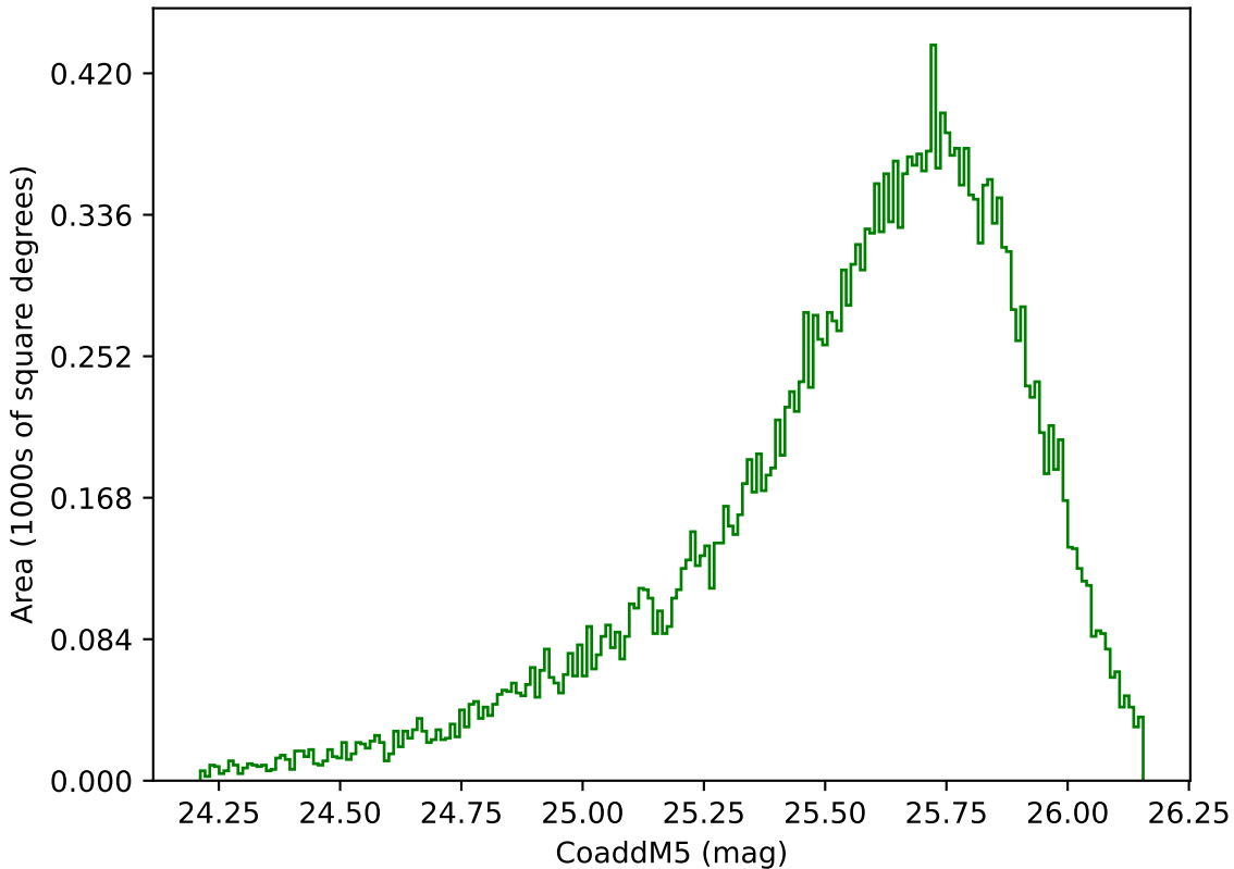
too_elab_r16_d3_gz_v3.4_10yrs Yr 1 g band: CoaddM5
