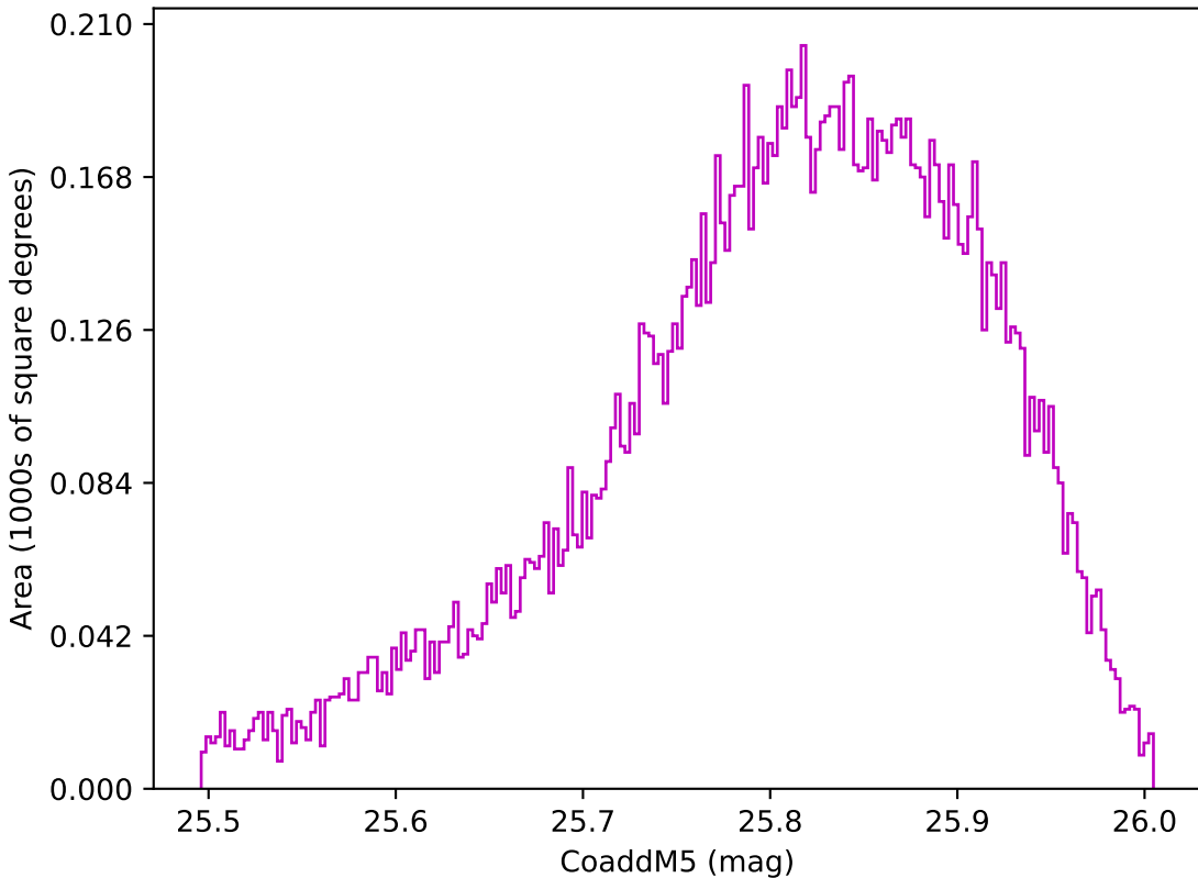
too_elab_r16_d3_gz_v3.4_10yrs WFD z band: CoaddM5
