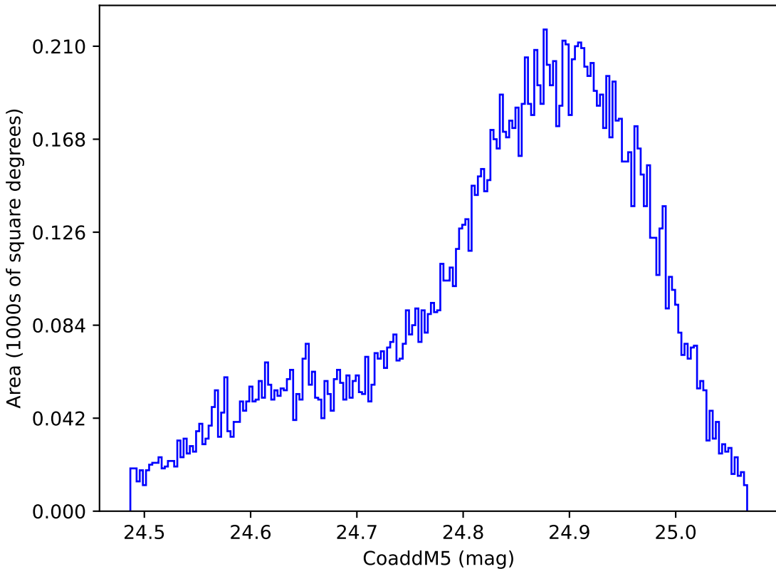
too_elab_r16_d3_gz_v3.4_10yrs WFD y band: CoaddM5
