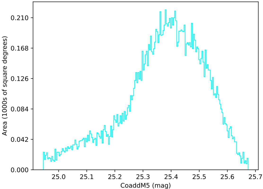
too_elab_r16_d3_gz_v3.4_10yrs WFD u band: CoaddM5
