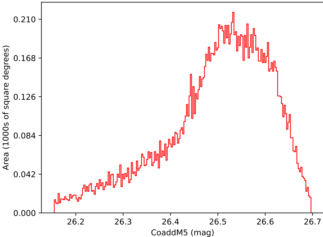
too_elab_r16_d3_gz_v3.4_10yrs WFD i band: CoaddM5
