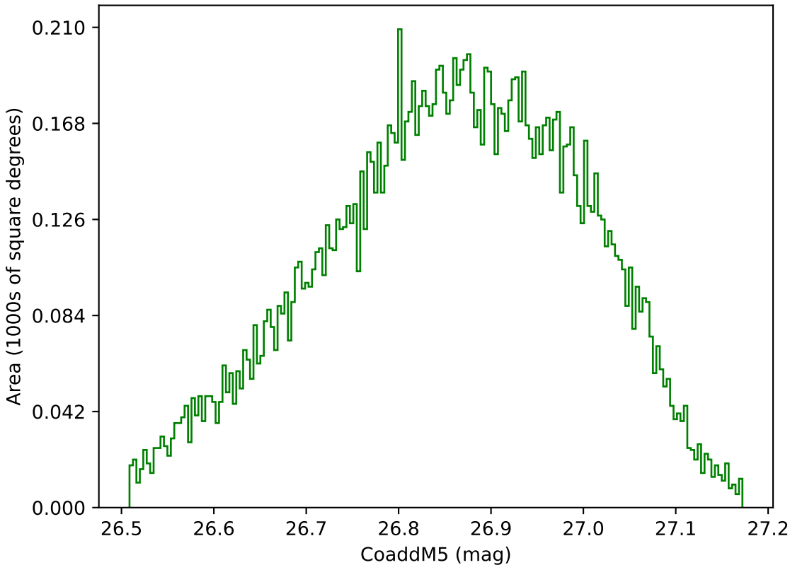
too_elab_r16_d3_gz_v3.4_10yrs WFD g band: CoaddM5
