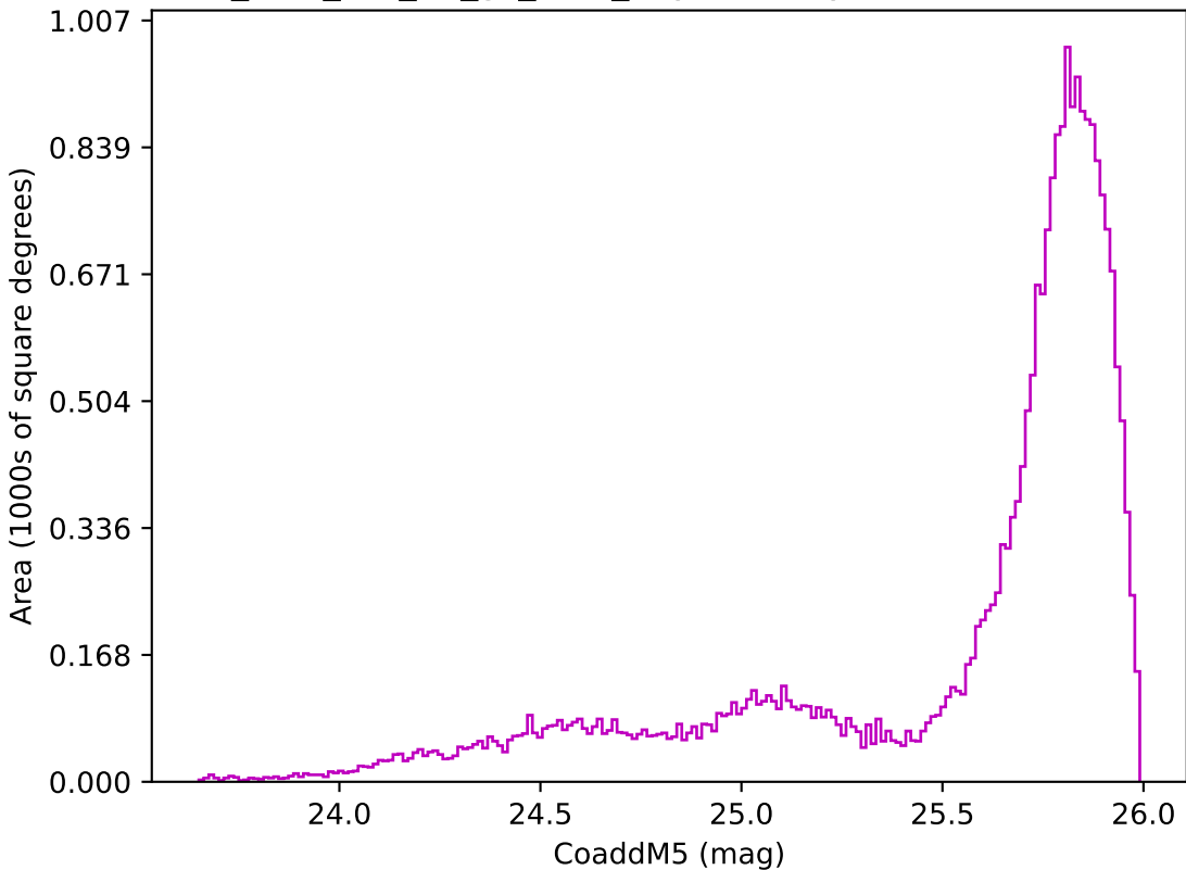
too_elab_r16_d3_gz_v3.4_10yrs All sky z band: CoaddM5
