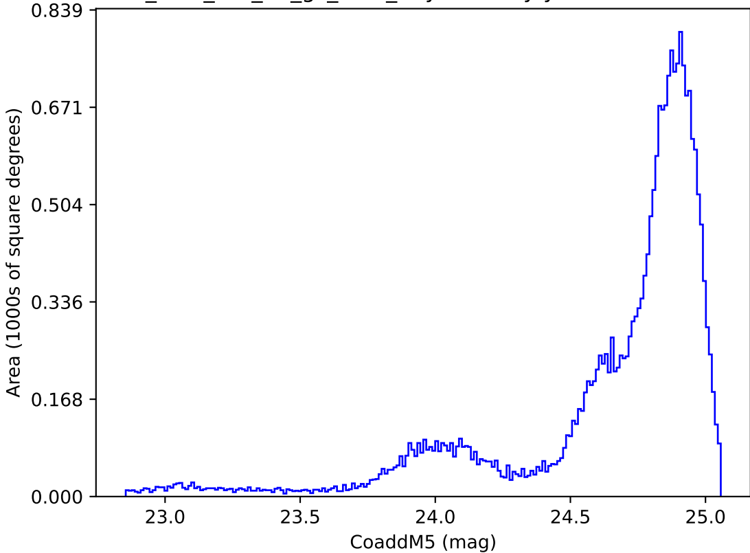
too_elab_r16_d3_gz_v3.4_10yrs All sky y band: CoaddM5
