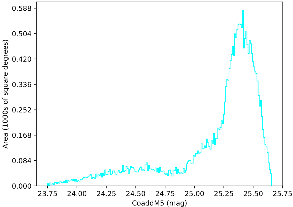
too_elab_r16_d3_gz_v3.4_10yrs All sky u band: CoaddM5
