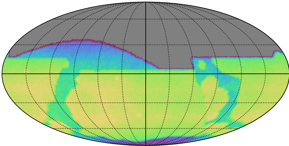
too_elab_r16_d3_gz_v3.4_10yrs All sky r band: CoaddM5
