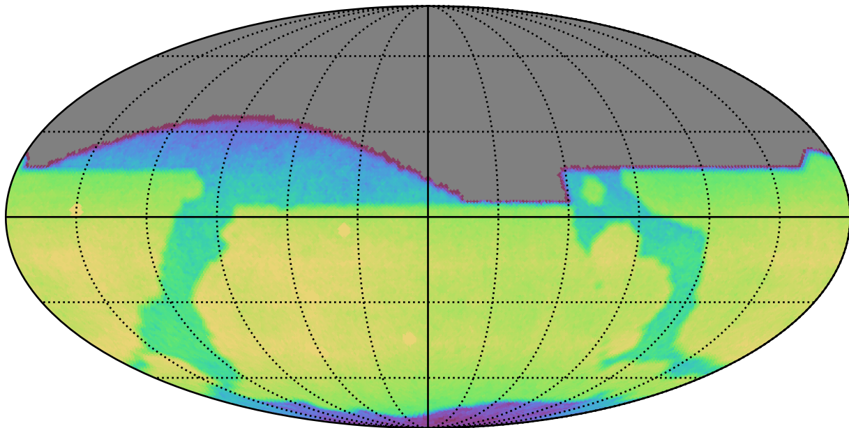
too_elab_r16_d3_gz_v3.4_10yrs All sky i band: CoaddM5
