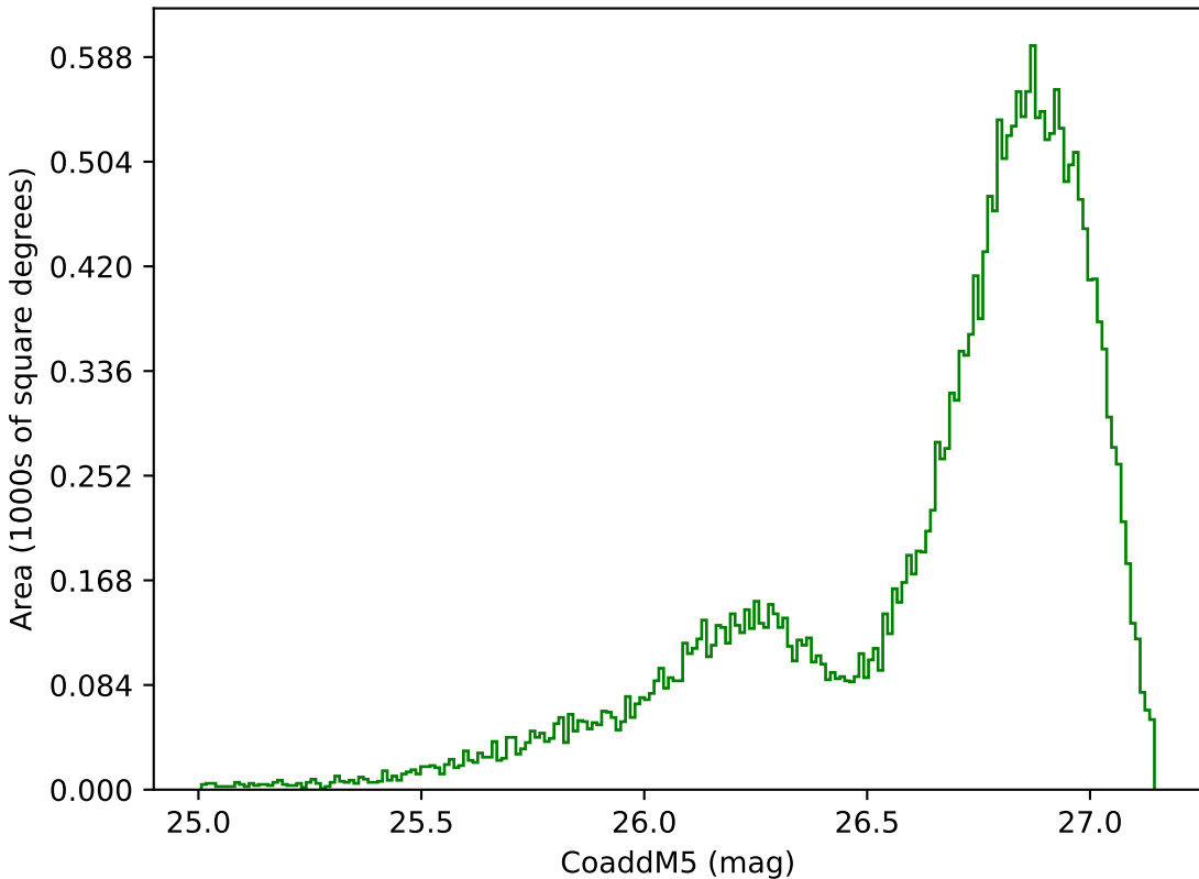
too_elab_r16_d3_gz_v3.4_10yrs All sky g band: CoaddM5
