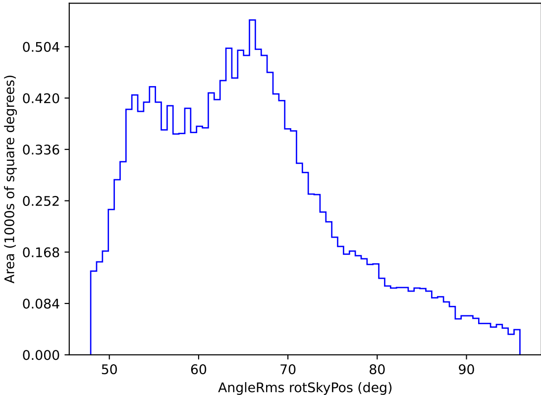
too_elab_r16_d3_gz_v3.4_10yrs WFD z band: AngleRms rotSkyPos
