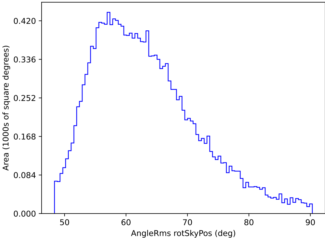
too_elab_r16_d3_gz_v3.4_10yrs WFD y band: AngleRms rotSkyPos
