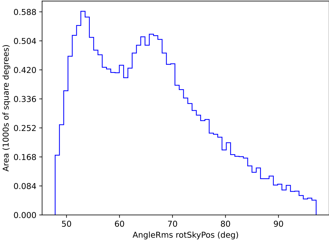
too_elab_r16_d3_gz_v3.4_10yrs WFD r band: AngleRms rotSkyPos
