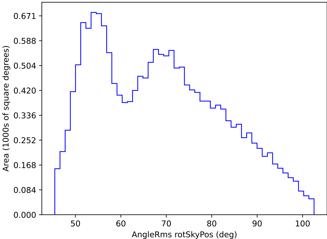
too_elab_r16_d3_gz_v3.4_10yrs WFD g band: AngleRms rotSkyPos
