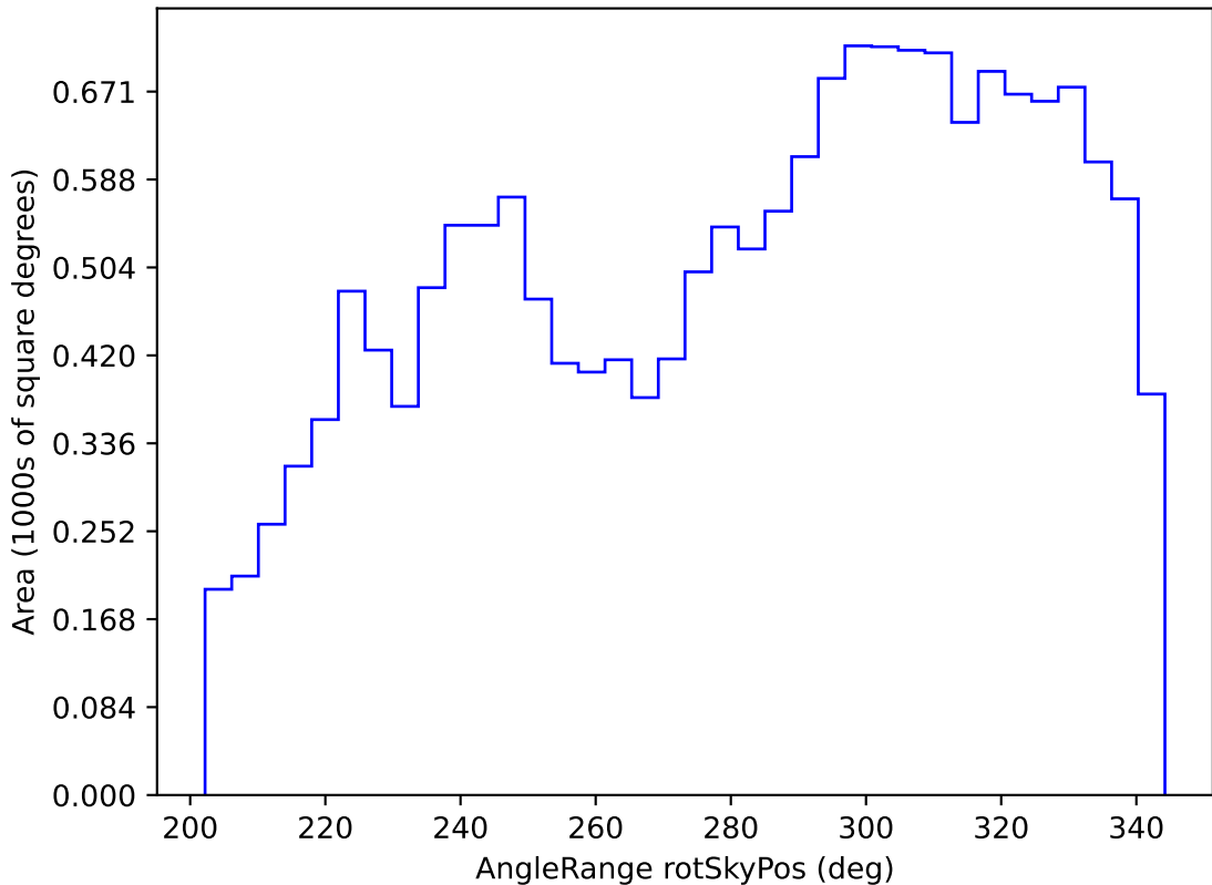
too_elab_r16_d3_gz_v3.4_10yrs WFD r band: AngleRange rotSkyPos
