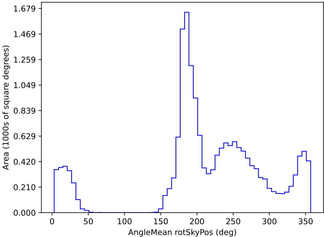
too_elab_r16_d3_gz_v3.4_10yrs WFD z band: AngleMean rotSkyPos
