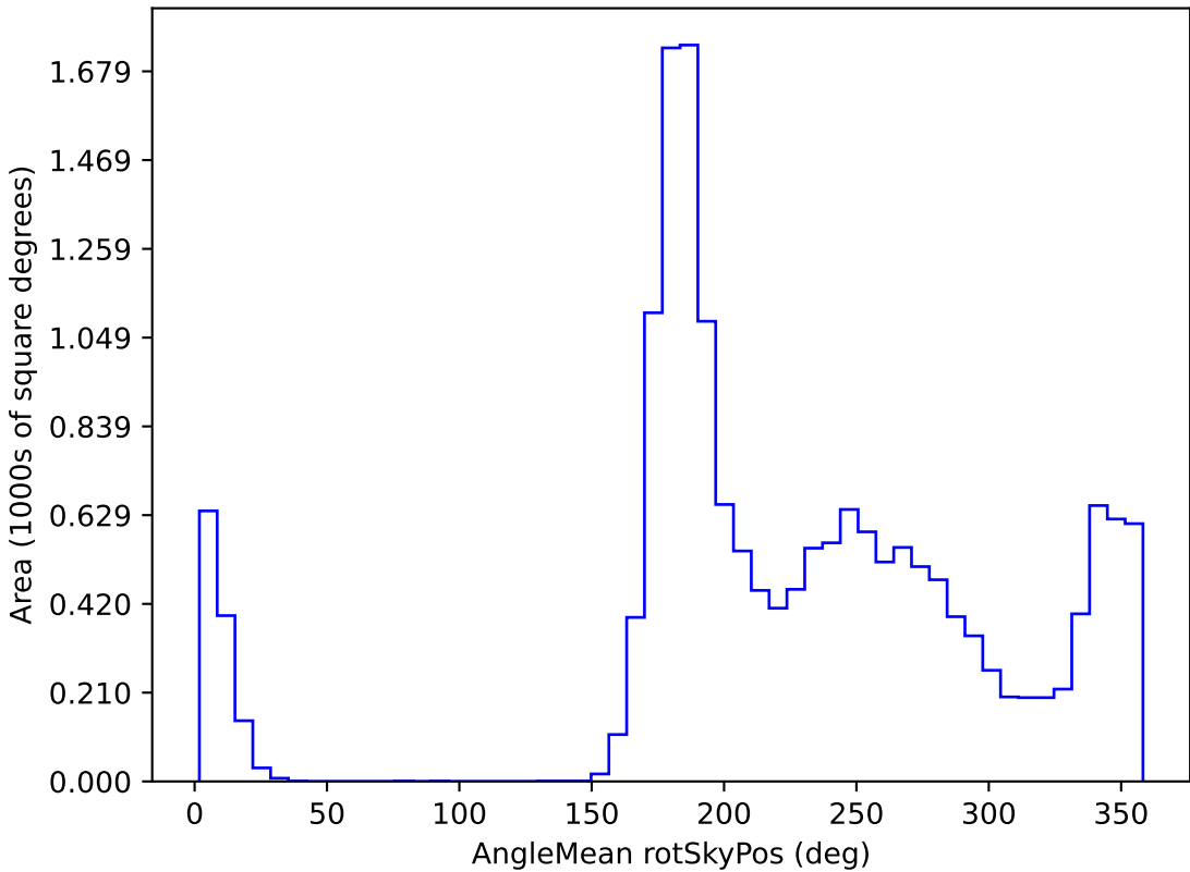
too_elab_r16_d3_gz_v3.4_10yrs WFD y band: AngleMean rotSkyPos
