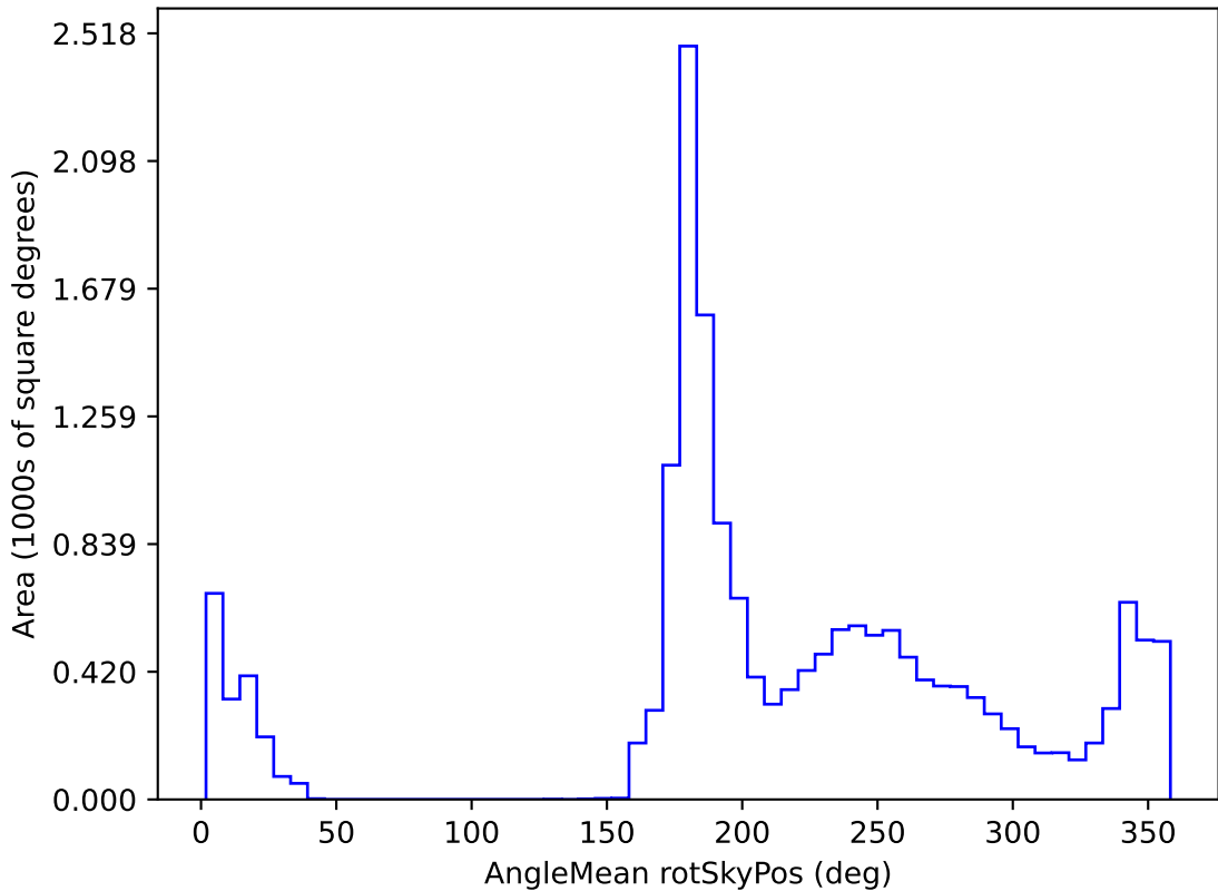
too_elab_r16_d3_gz_v3.4_10yrs WFD all bands: AngleMean rotSkyPos
