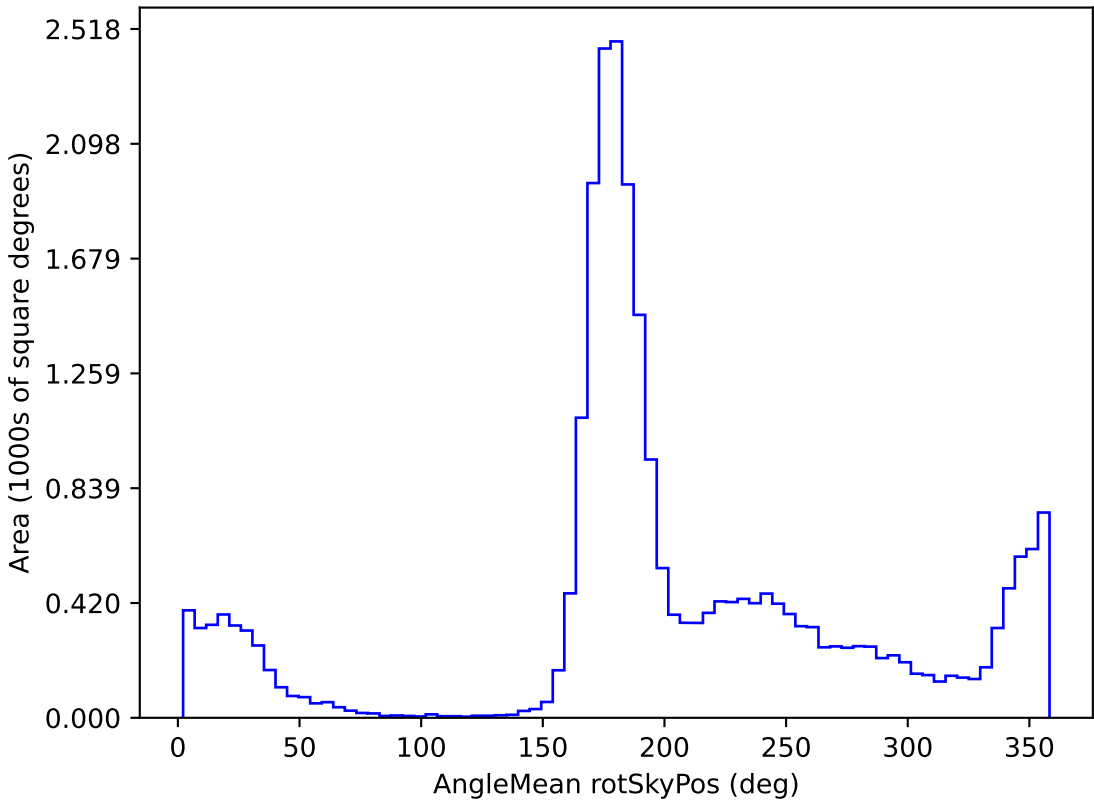
too_elab_r16_d3_gz_v3.4_10yrs All sky r band: AngleMean rotSkyPos
