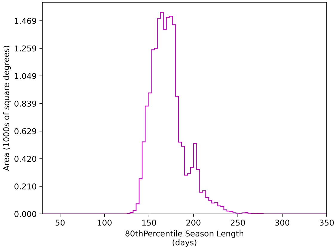
too_elab_r16_d3_gz_v3.4_10yrs WFD z band: 80thPercentile Season Length
