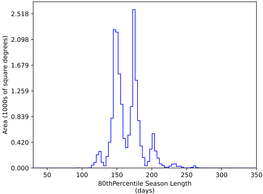
too_elab_r16_d3_gz_v3.4_10yrs WFD y band: 80thPercentile Season Length
