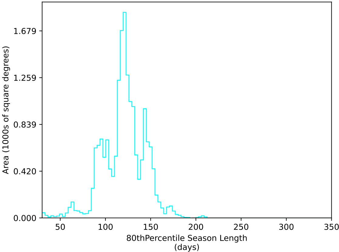
too_elab_r16_d3_gz_v3.4_10yrs WFD u band: 80thPercentile Season Length
