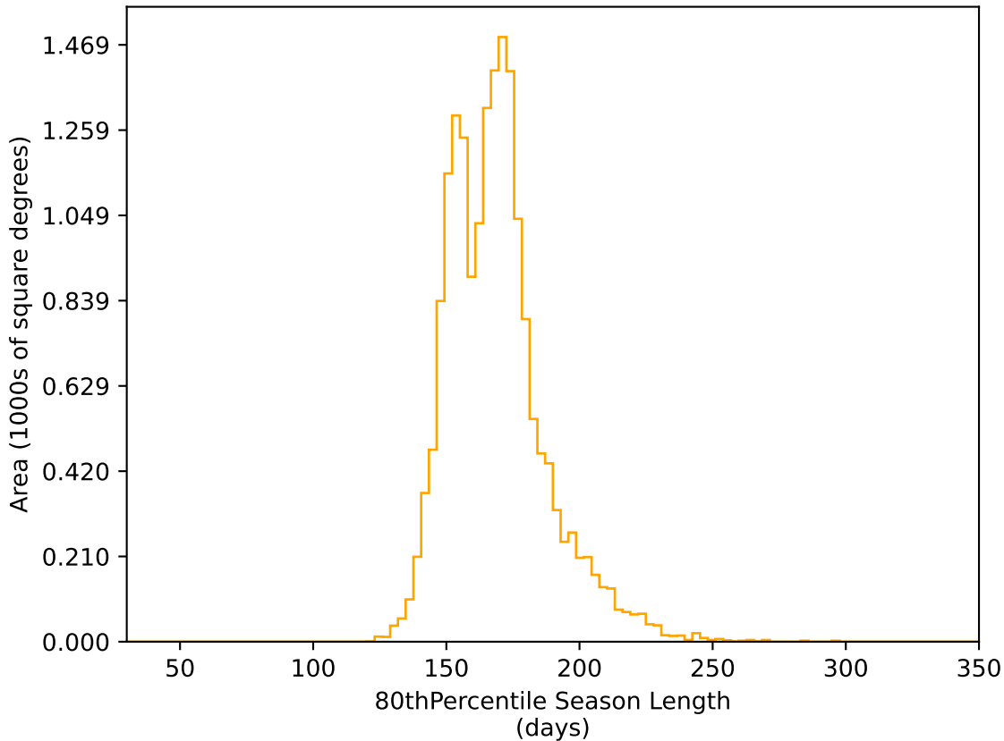
too_elab_r16_d3_gz_v3.4_10yrs WFD r band: 80thPercentile Season Length
