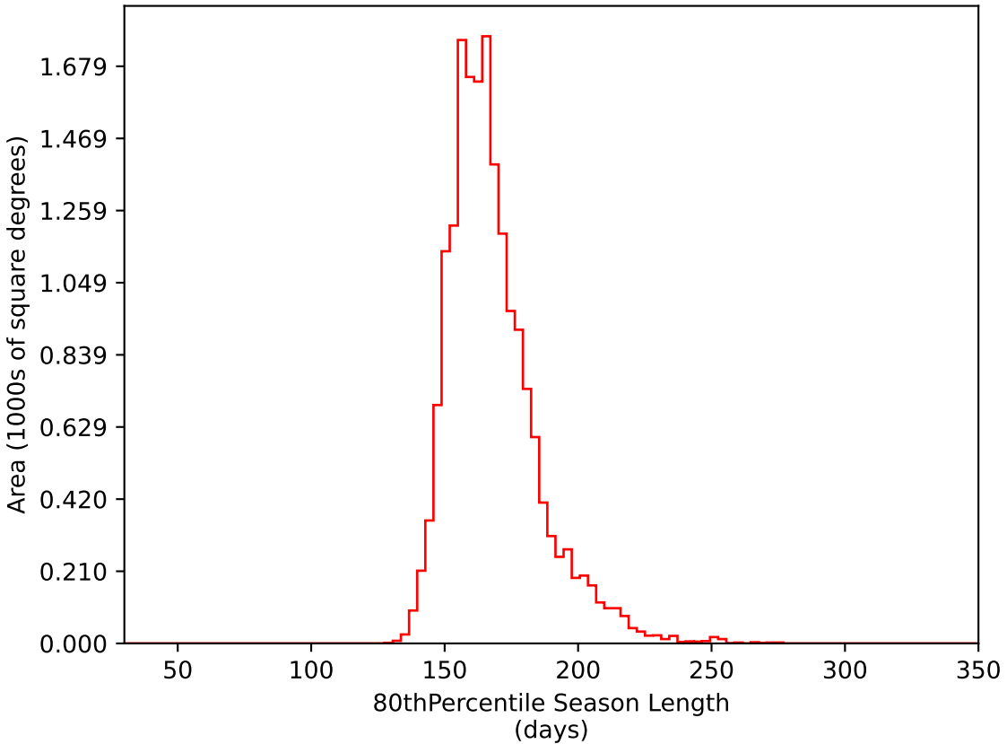
too_elab_r16_d3_gz_v3.4_10yrs WFD i band: 80thPercentile Season Length
