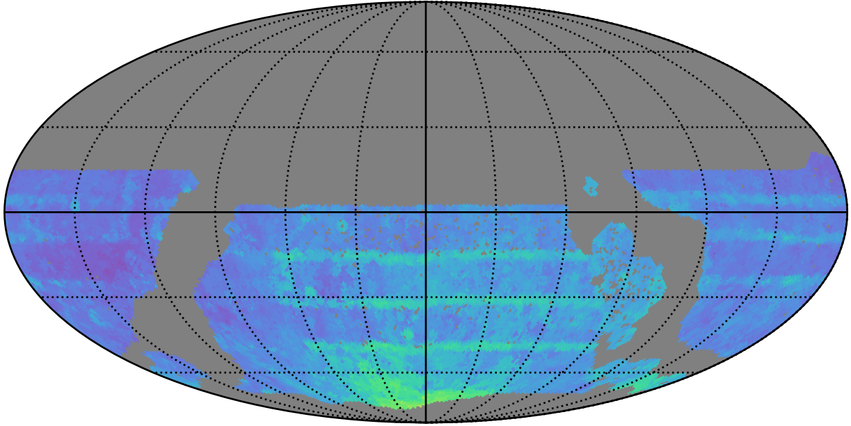
too_elab_r16_d3_gz_v3.4_10yrs WFD all bands: 80thPercentile Season Length
