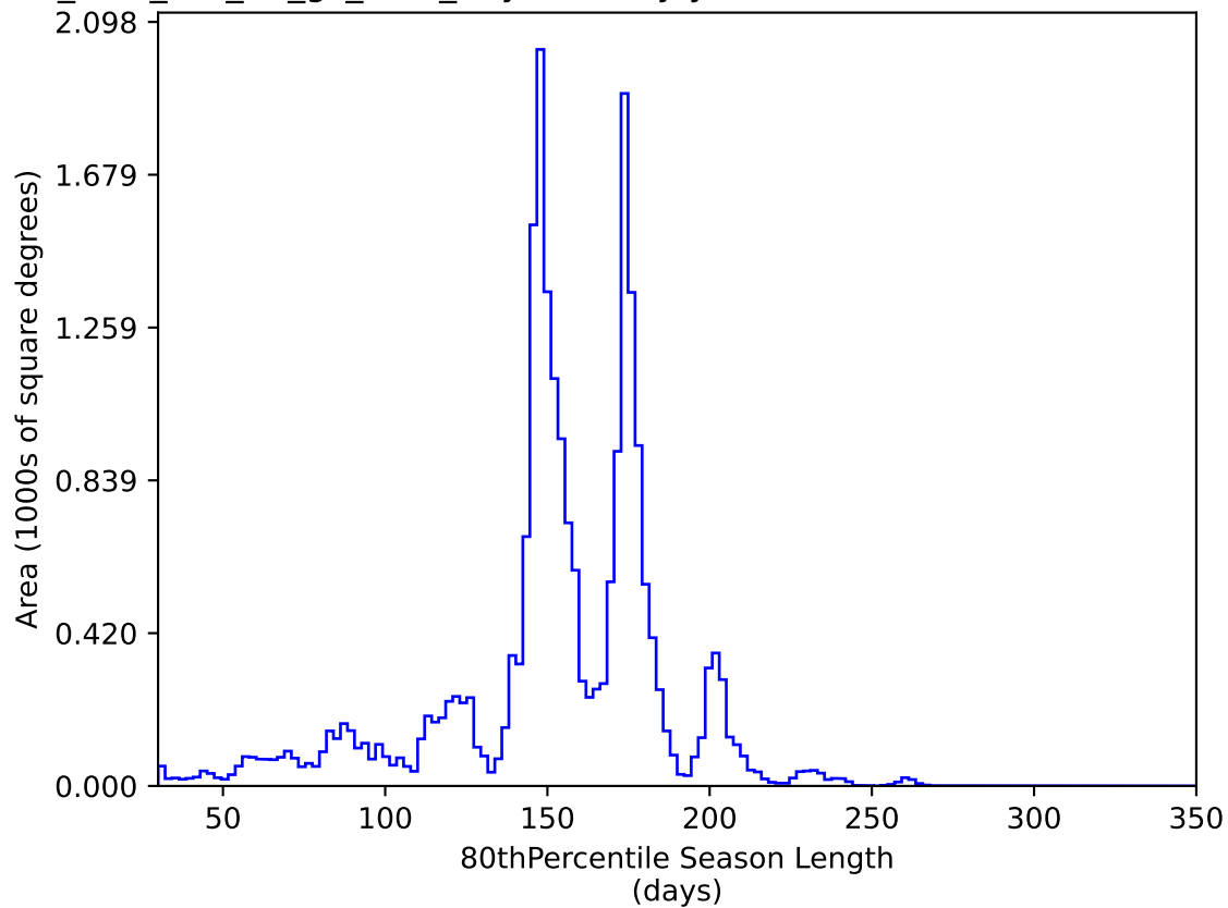
too_elab_r16_d3_gz_v3.4_10yrs All sky y band: 80thPercentile Season Length
