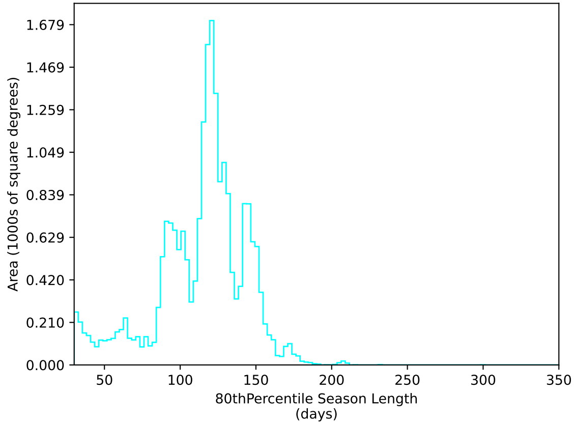
too_elab_r16_d3_gz_v3.4_10yrs All sky u band: 80thPercentile Season Length
