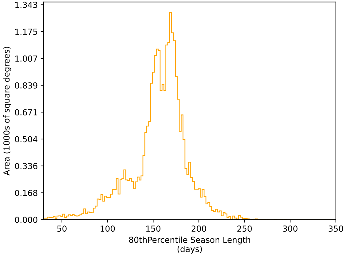
too_elab_r16_d3_gz_v3.4_10yrs All sky r band: 80thPercentile Season Length
