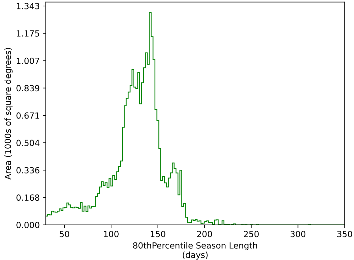
too_elab_r16_d3_gz_v3.4_10yrs All sky g band: 80thPercentile Season Length
