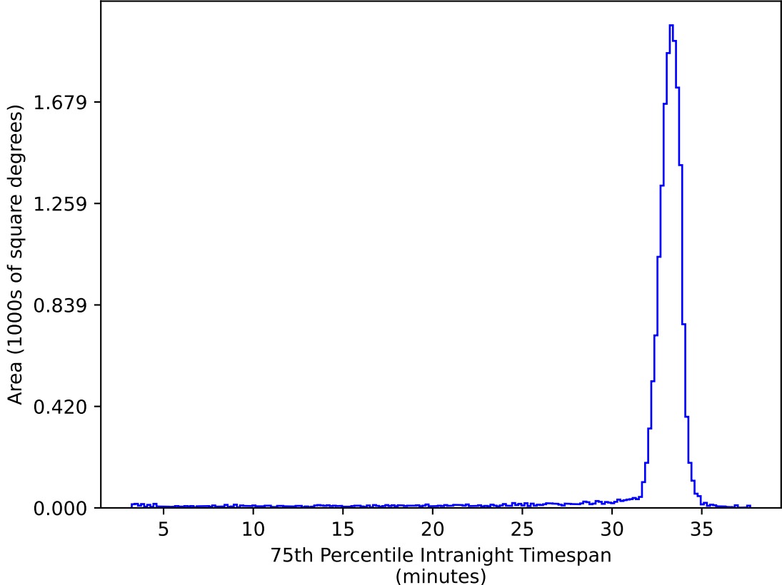
too_elab_r16_d3_gz_v3.4_10yrs WFD ug bands: 75th Percentile Intranight Timespan
