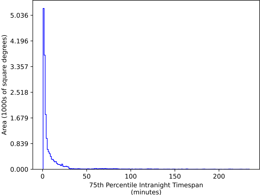
too_elab_r16_d3_gz_v3.4_10yrs WFD u band: 75th Percentile Intranight Timespan
