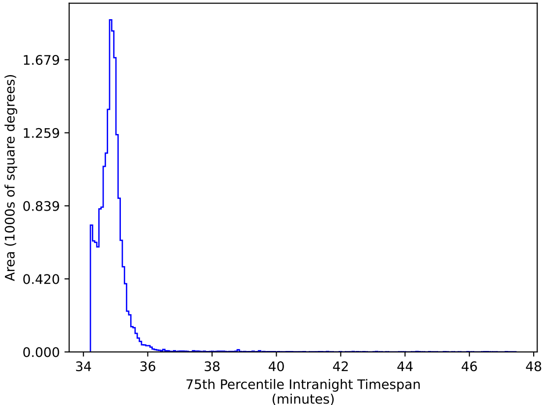
too_elab_r16_d3_gz_v3.4_10yrs WFD iz bands: 75th Percentile Intranight Timespan
